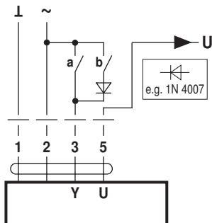
Position control: 90^\circ = 100s Flow control: V_{max} = 100s
